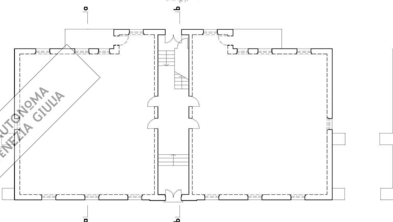
pianta piano terra ground floor plan
