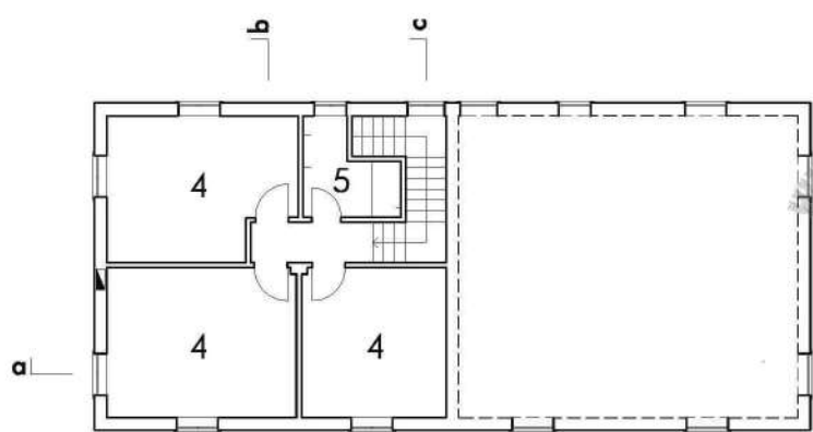
pianta piano primo first floor plan
